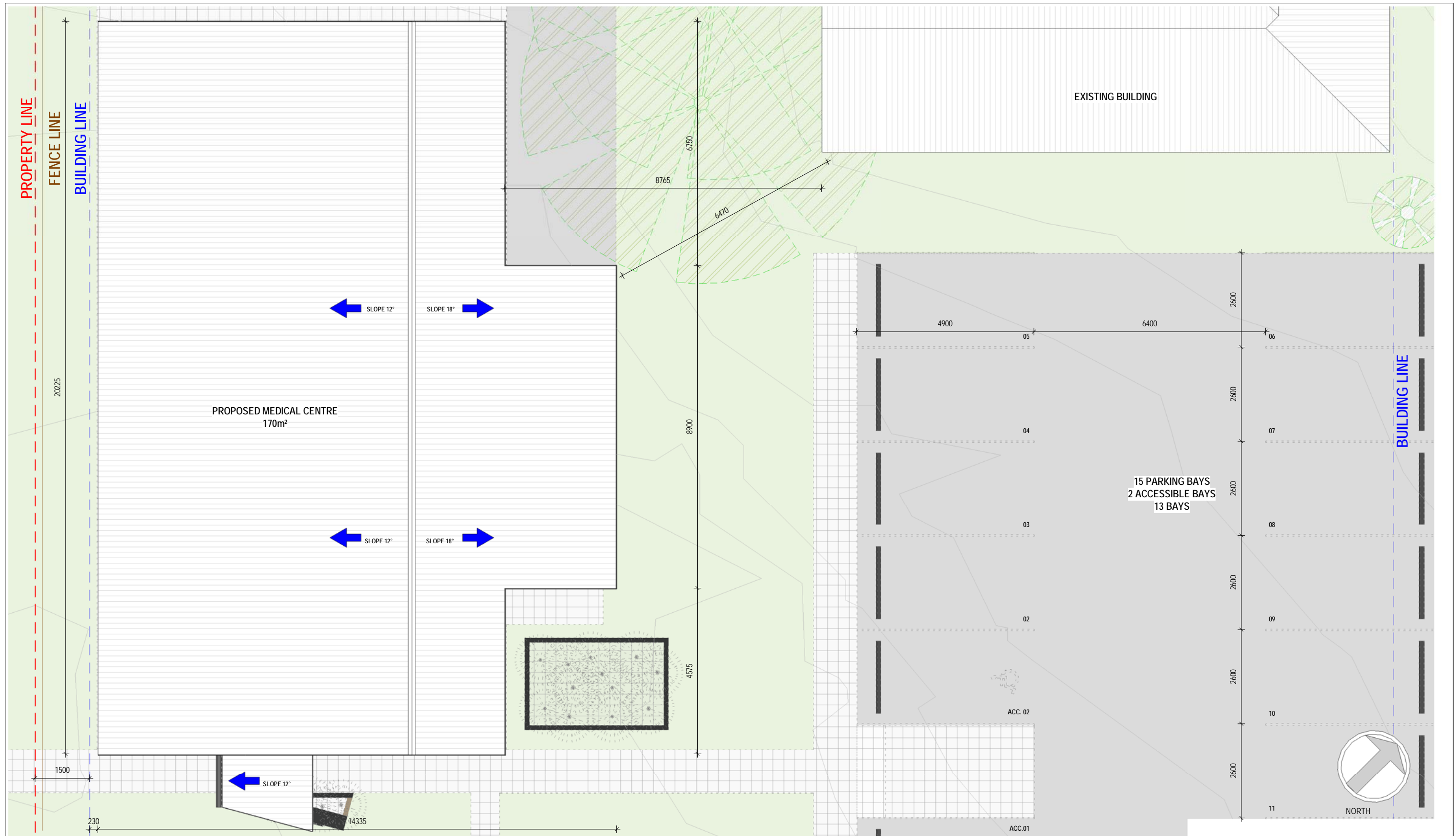
1 TPA-004. Roof Plan Scale: 1 : 100
